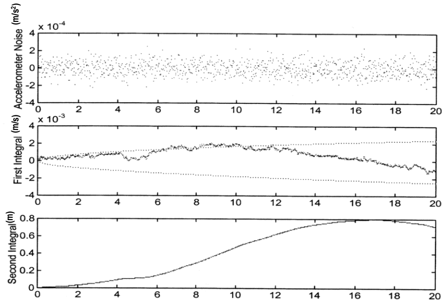
Figure 1.2. Accelerometer noise and its first two integrals.
